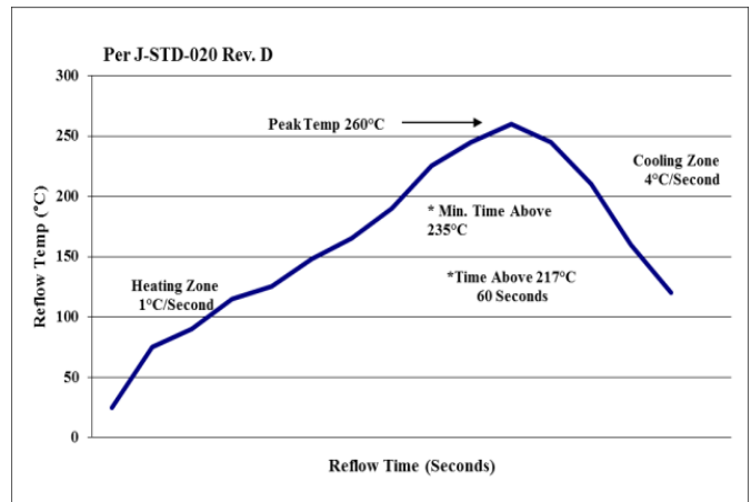
Figure 23. Recommended linear reflow profile using Sn/Ag/Cu solder.
