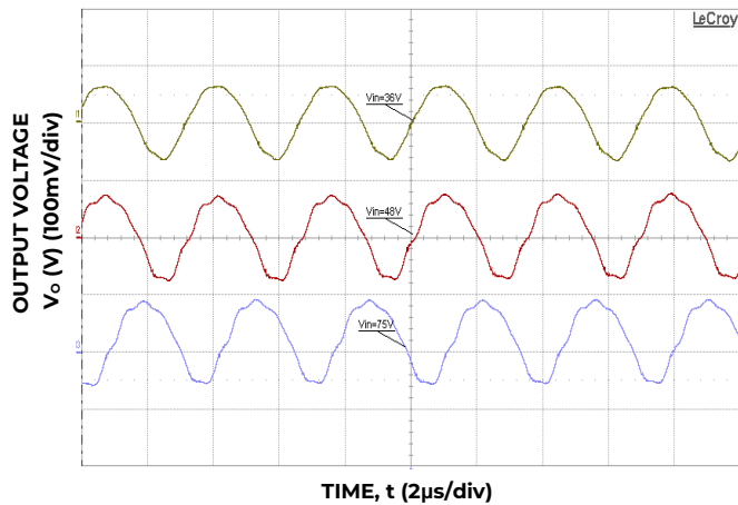
Figure 2. Typical output ripple and noise ( I_o = I_{o, max} ).
