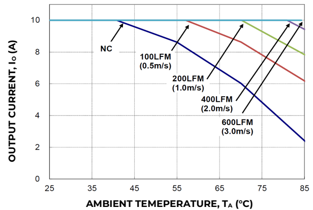
Figure 16. Output Current Derating for the Module with Heatplate; Airflow in the Transverse Direction from V_{out}(-) to V_{out}(+) ; V_{IN}=48V , V_O=12V .
