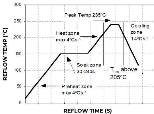
Figure 21. Reflow Profile for Tin/Lead (Sn/Pb) process.
