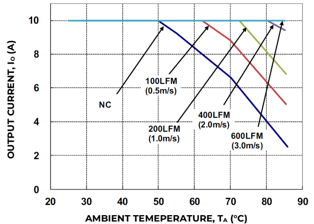
Figure 17. Output Current Derating for the Module with -18H Heatplate; Airflow in the Transverse Direction from V_{out}(-) to V_{out}(+) ; V_{IN}=48V , V_O=12V .
