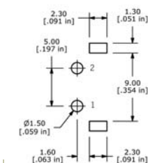
P.C. MOUNTING
