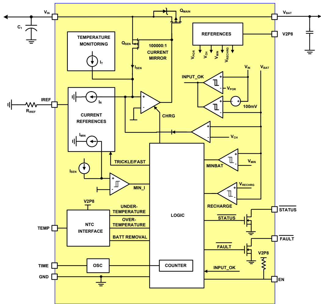
FIGURE 3. BLOCK DIAGRAM
