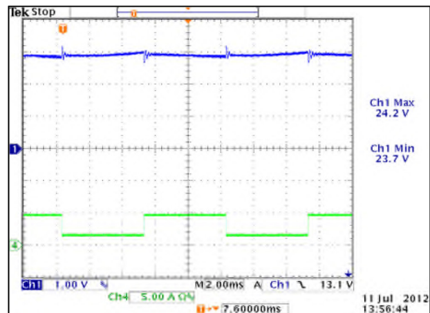
240Vac Input, 24V Output, 25% to 75% Load Step
