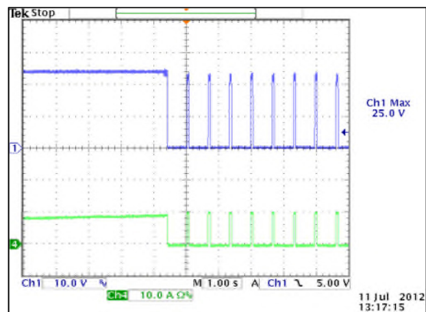
264Vac Input, 24V Output
