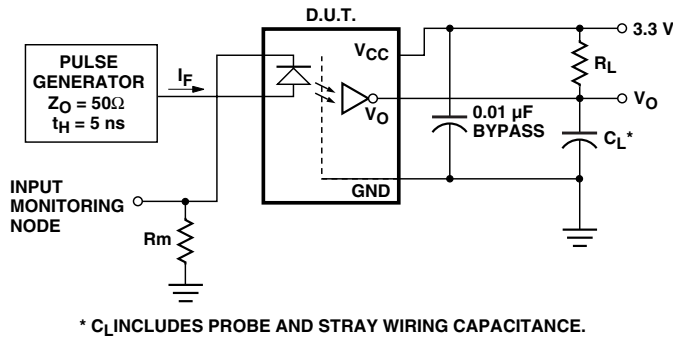
Figure 4: Test Circuit for t_{PHL} and t_{PLH}
