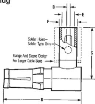
Plug
