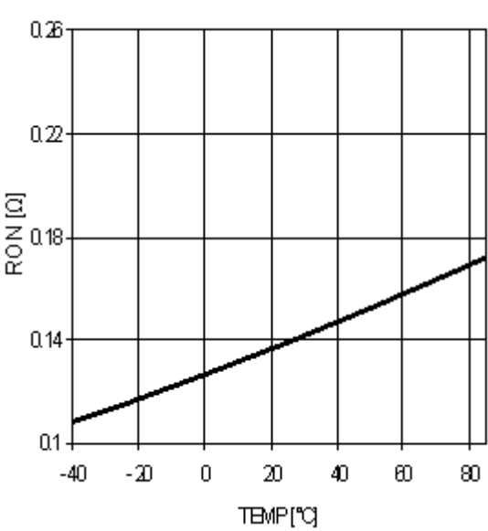
Fig.8 Hi,Low-Side On-resistance
