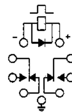
TERMINAL VIEW
