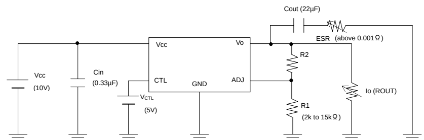
※Operation Note 11 Measurement circuit
