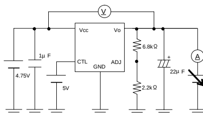
Measurement Circuit of Fig.6
