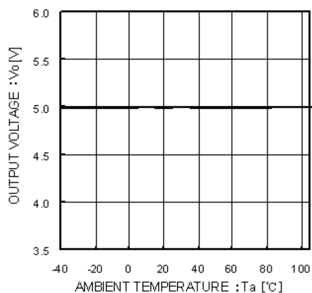
Fig.8 Output Voltage
