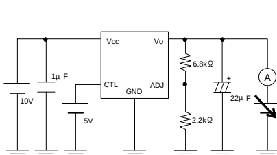
Measurement Circuit of Fig.5
