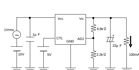
Measurement Circuit of Fig.7
