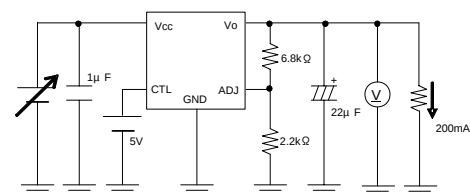
Measurement Circuit of Fig.4
