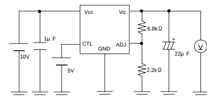
Measurement Circuit of Fig.13
