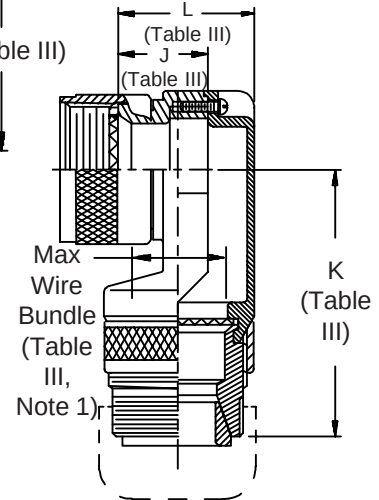
Ultra Low-Profile Split 90°
