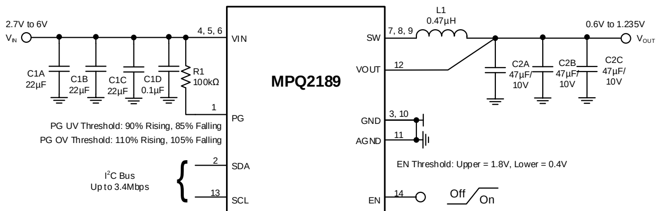
Figure 3: Typical Application Circuit ( f_{sw} = 1.25\text{MHz} , V_{OUT} = 0.8\text{V} , FCCM)
