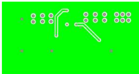
Mid-Layer 2
