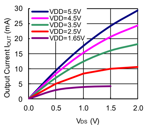
14) Pch Driver Output Current vs. V_{\text{DS}}
