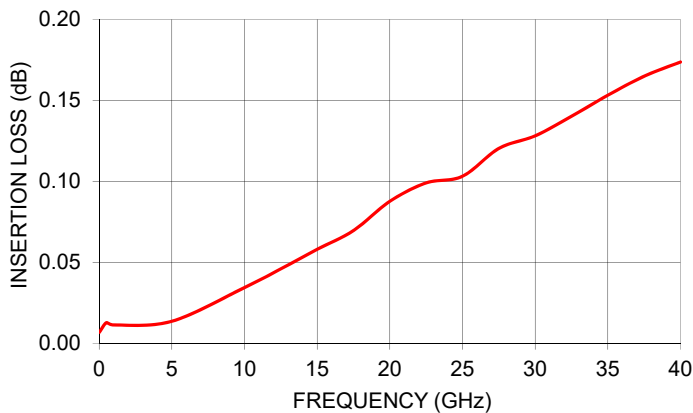
KM-24M+ INSERTION LOSS
