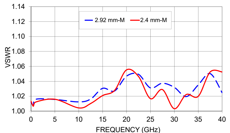
KM-24M+ VSWR
