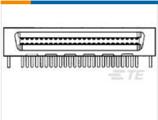
TE Part #1734037-2 Champ 050 series,80pos,Au over PdNi
