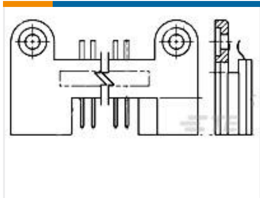
TE Part #583580-1 BOX PIN 50 POS. 100 C/L
