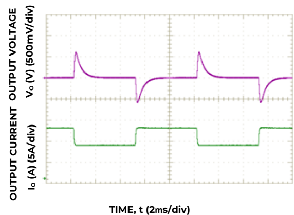
Figure 6. Dynamic Load Change Transient Response from 50 % to 75% to 50% of Full Load at Room Temperature and 48V_{in} ; 0.1A/uS , C_{o,ext} = 440\mu F .
