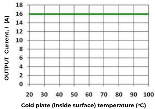
Figure 18. Power Derating for JRCW016A0R in Conduction cooling (cold plate) applications; T_a < 70^\circ\text{C} adjacent to module; V_{IN} = V_{IN,NOM}
