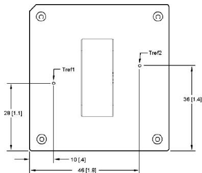
Figure 17. Case 17. Case (T REF ) Temperature Measurement Location (top view).
