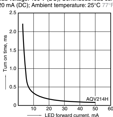
10-(2). Turn on time vs. LED forward current characteristics
