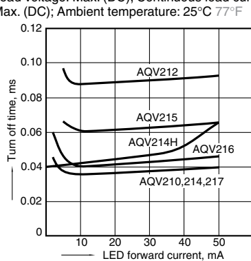
11. Turn off time vs. LED forward current characteristics
