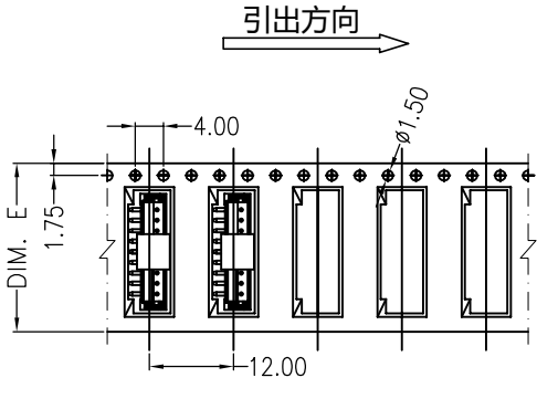
02~08 CONTACTS
