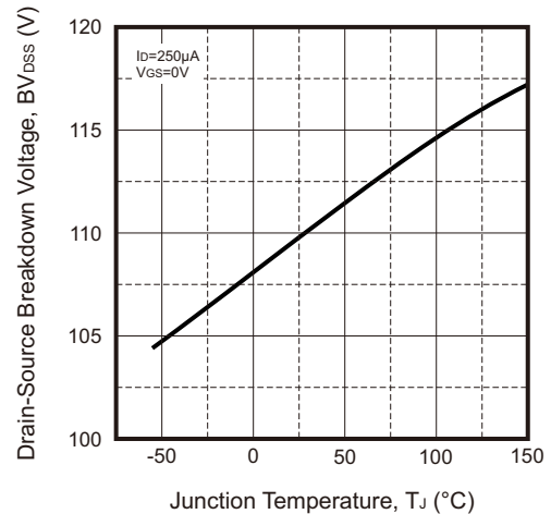
Fig.4 - Drain-Source Breakdown Voltage
