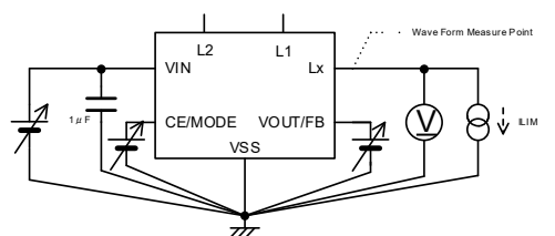
< Circuit No.6 >
