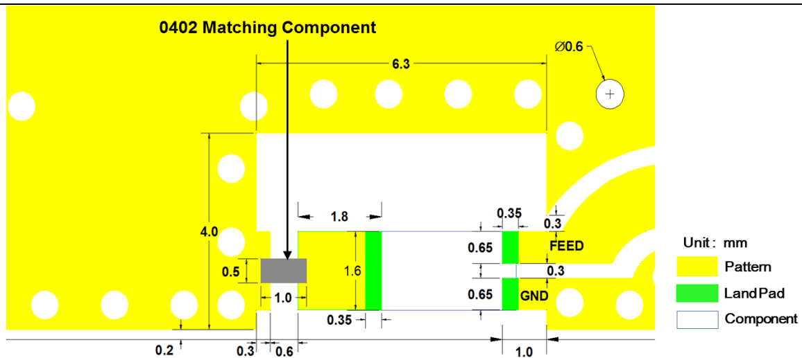
Land Pattern
