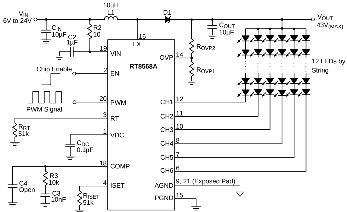
Figure 2. Application Circuit 2
