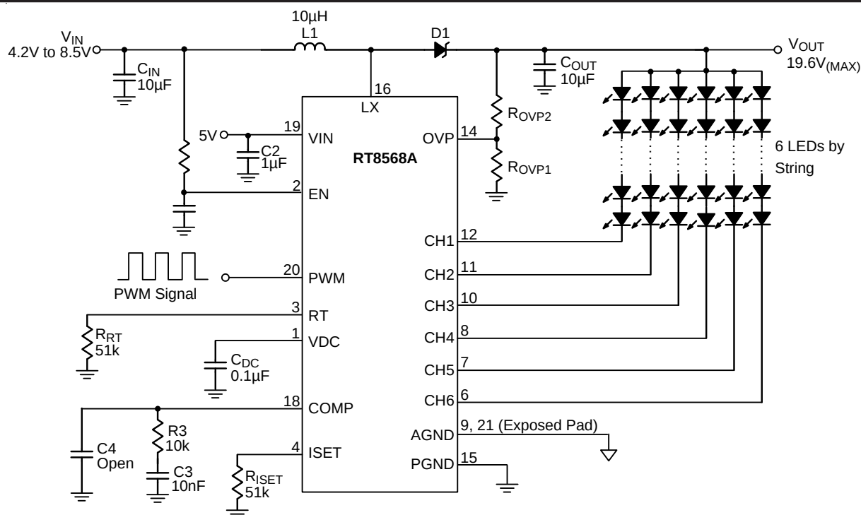
Figure 3. Application Circuit 3
