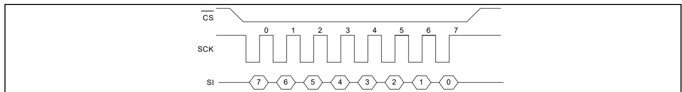
Figure 5 SPI mode 3
