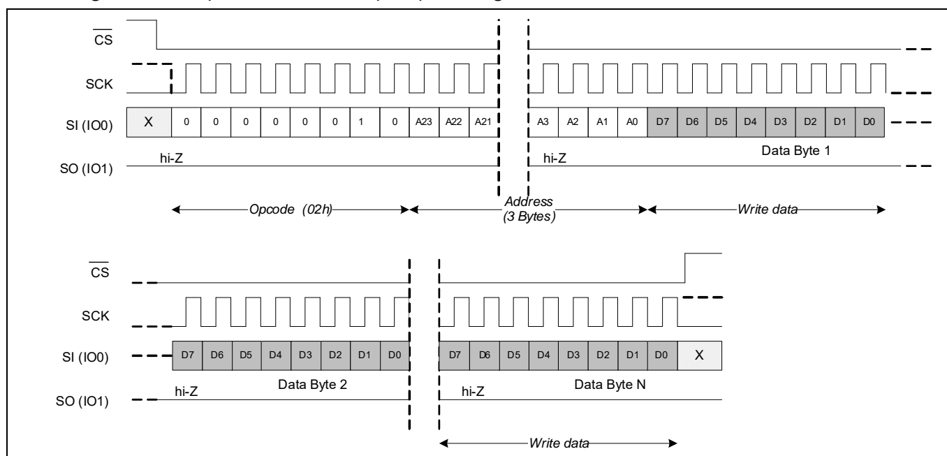
Figure 39 Memory write (WRITE) in SPI mode
