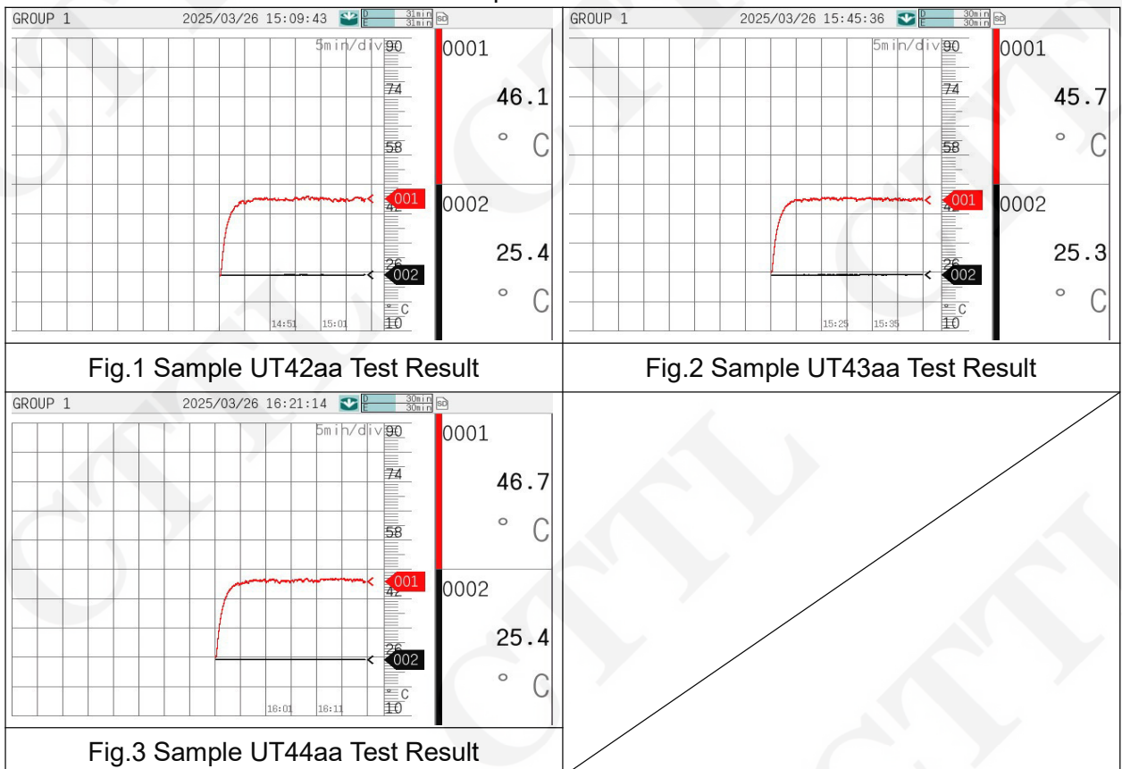
B-6 Temperature Rise Curve
