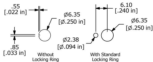
PANEL MOUNTING
