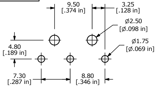
P.C. MOUNTING
