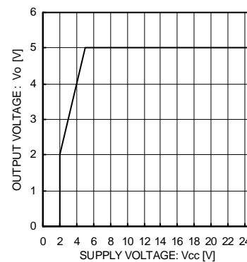
Fig.15 Line Regulation ( I_o=0\text{mA} )
