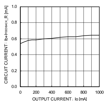
Fig.9 Circuit Current ( I_o=0\text{mA} \rightarrow 1000\text{mA} )
