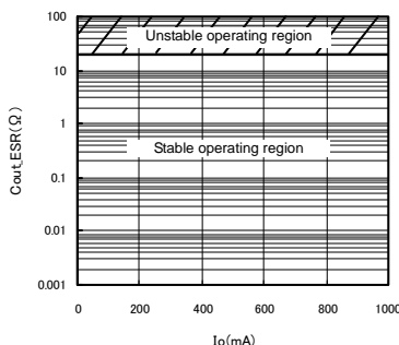
Cout_ESR vs Io(reference data)
