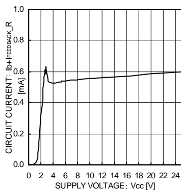
Fig.1 Circuit Current
