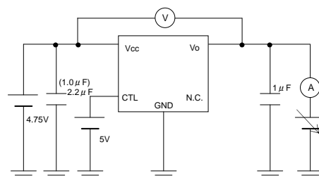
Measurement Circuit of Fig.6 and Fig.18
