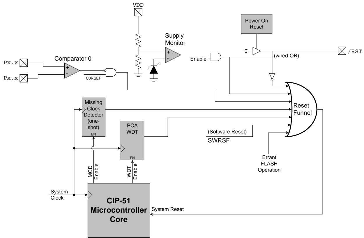
Figure 10.1. Reset Sources
