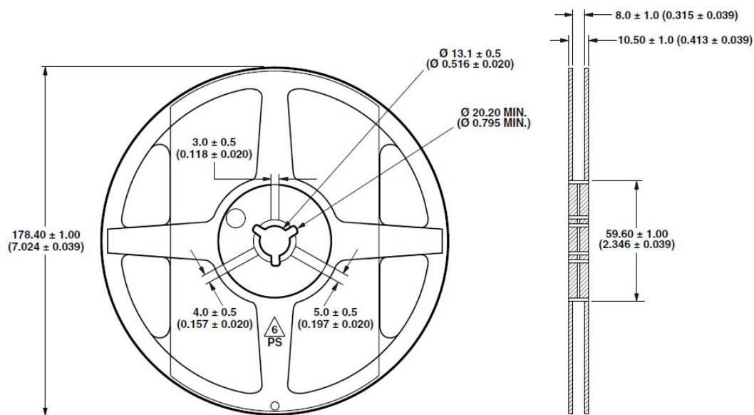
Figure 8: Reel Dimensions
