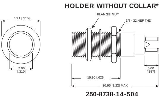
HOLDER WITHOUT COLLAR*
