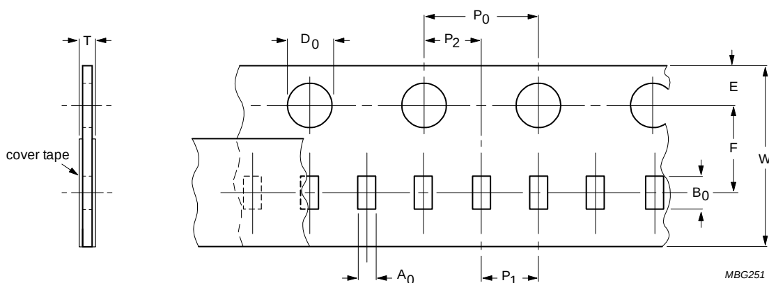
Fig. 14 Paper/PE Tape
