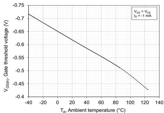
Figure 59. Gate Threshold Voltage vs. Ambient Temperature
