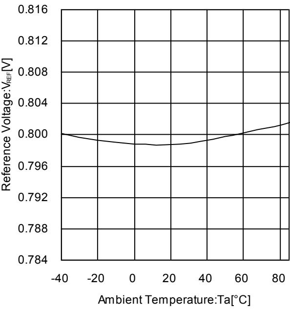
Figure 37. REG3 Reference Voltage vs Temperature
