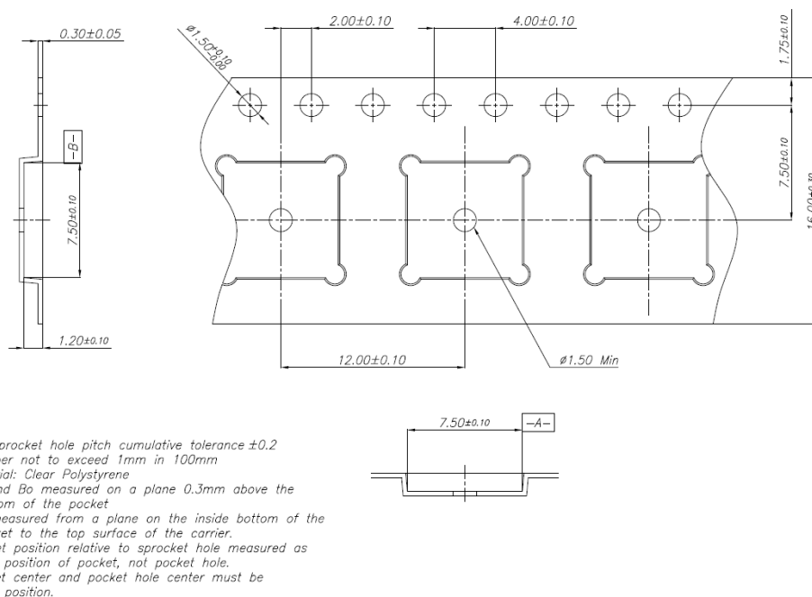
Figure 6: EVA-M8M/Q tape dimensions
