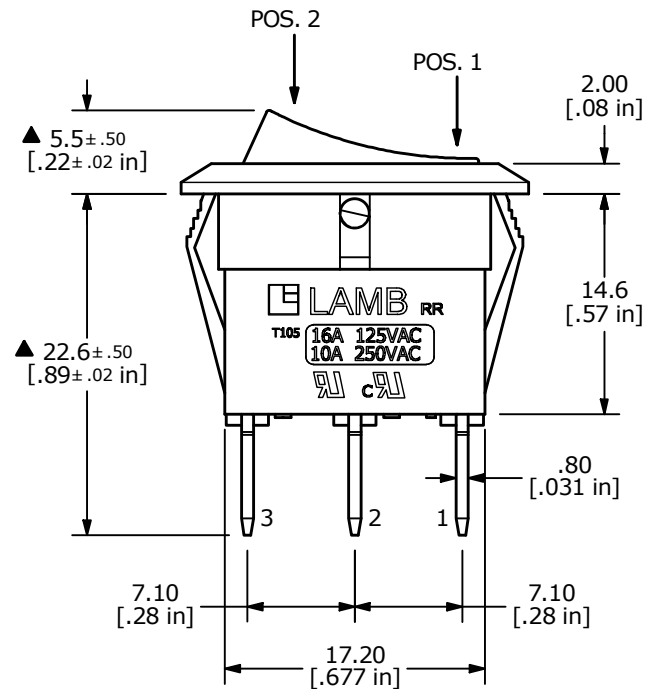
CIRCUIT: SPST
