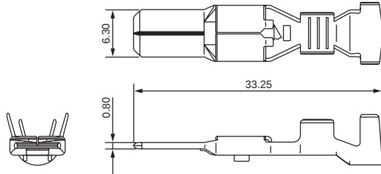
Male Terminal
