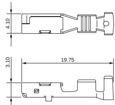
Female Terminal
