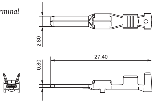
Female Terminal
