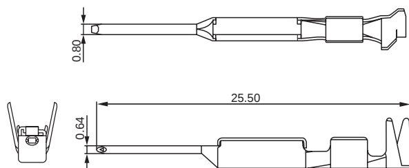
Male Terminal
