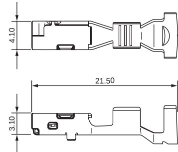
Female Terminal
