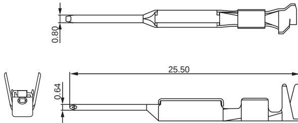
Male Terminal
