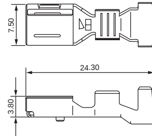
Female Terminal
