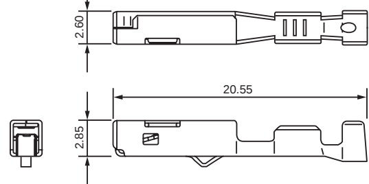
Female Terminal
