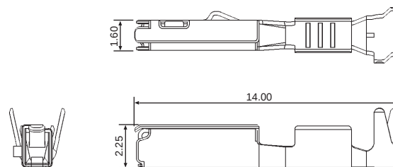
Female Terminal
