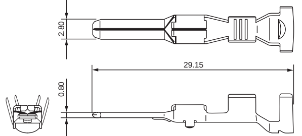
Male Terminal
