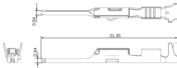
Male Terminal
