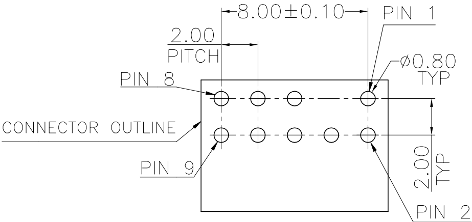
5 RECOMMENDED PCB LAYOUT TOLERANCE ± 0.05 (TOP VIEW)
