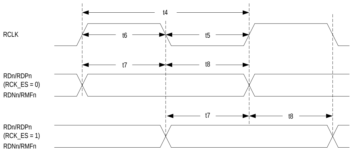
Figure-48 Receive Clock Timing Diagram
