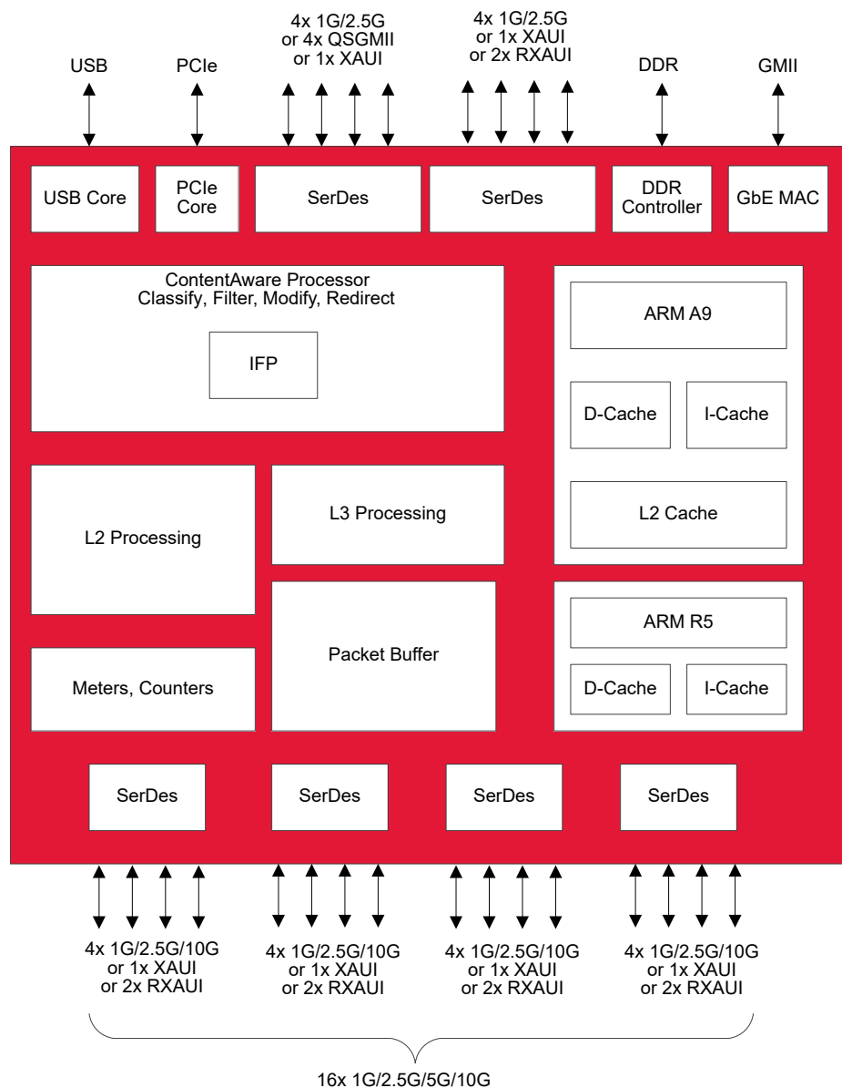
Figure. BCM5340X/BCM5341X Block Diagram
