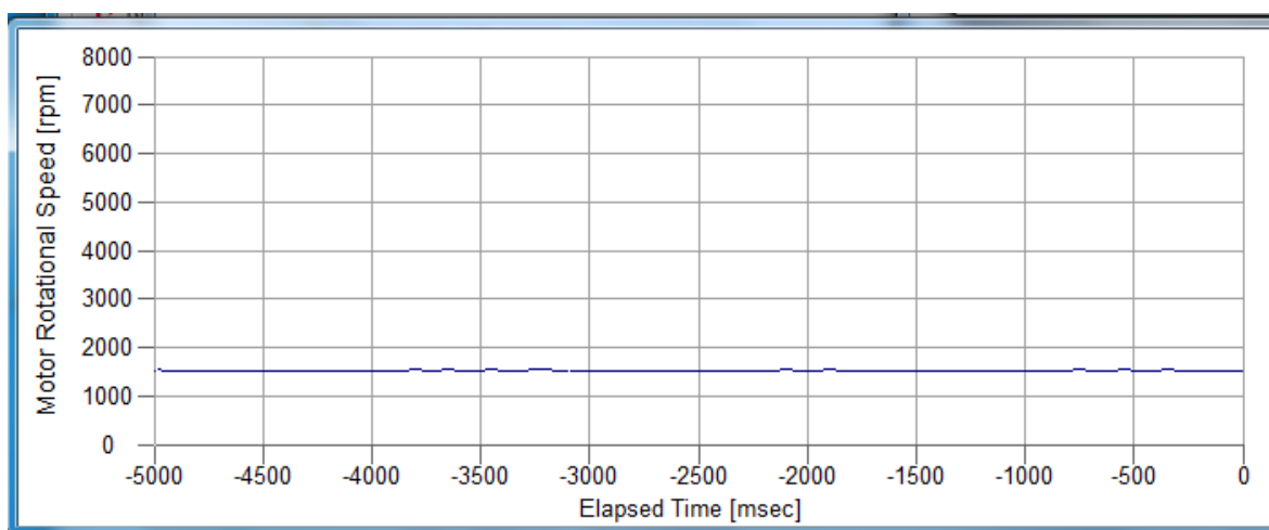
Figure 15. Graph window
