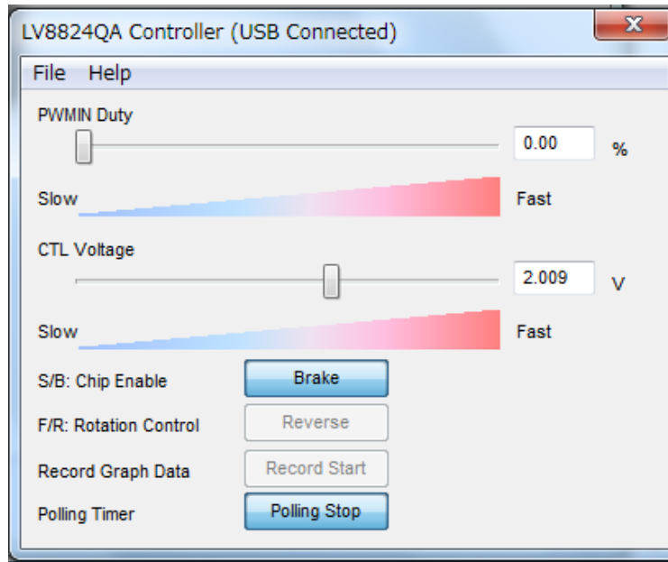
Figure 16. Controller window 1-1
