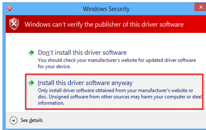
Figure 10. Windows Security
