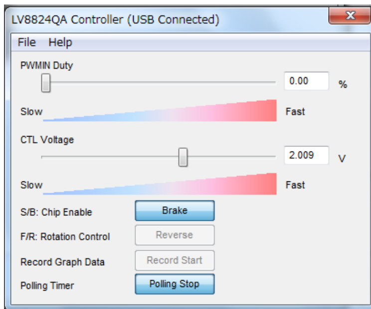
Figure 13. Controller window
