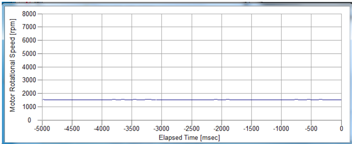
Figure 19. Graph window
