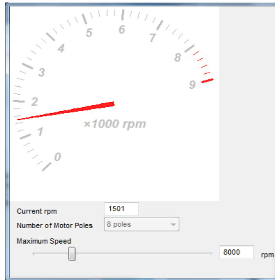
Figure 18. Tachometer window
