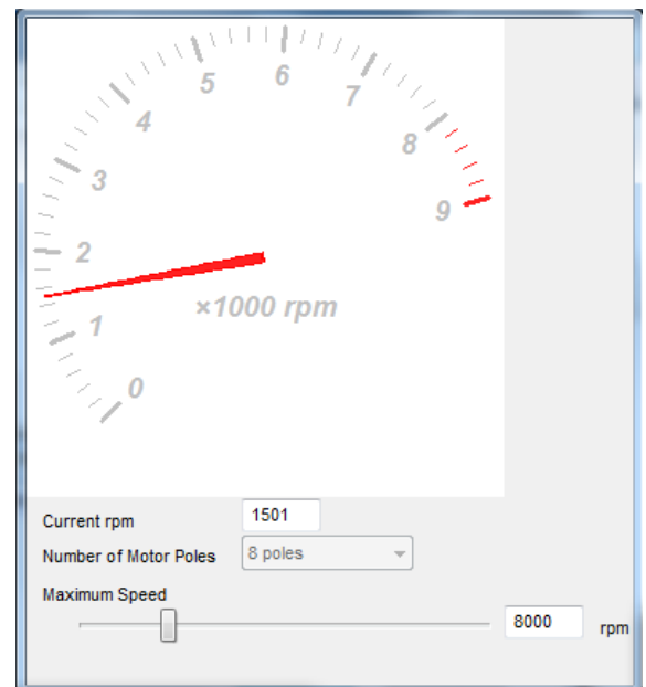
Figure 14. Tachometer window
