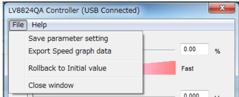
Figure 17. controller window 1-2
