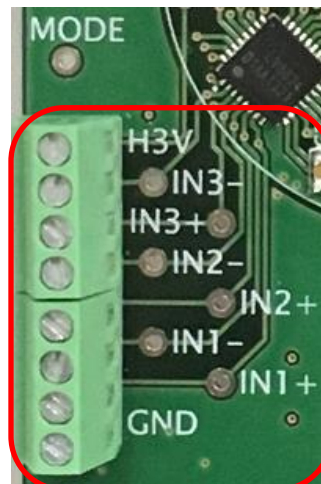
Figure 4. Hall sensor connector
