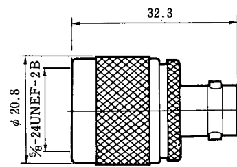
UG-201A/U CL311-0007-8
