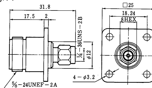
HRM-557S CL311-0138-6
