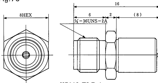
HRMJ-FLP-1 CL311-0195-0
