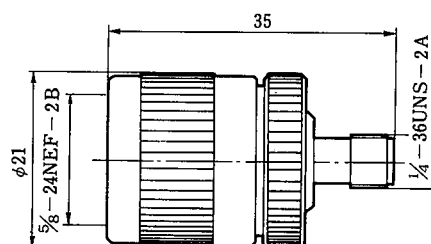
HRM-508 (09) CL311-0092-7-09
