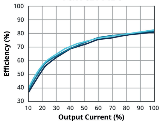
EFFICIENCY VS OUTPUT LOAD PCN1-S24-D12-S
