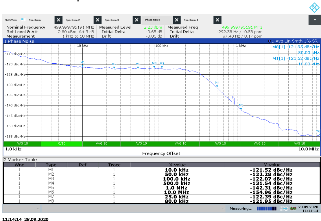
Figure 16 Typical Phase Noise at 500 MHz RF Output
