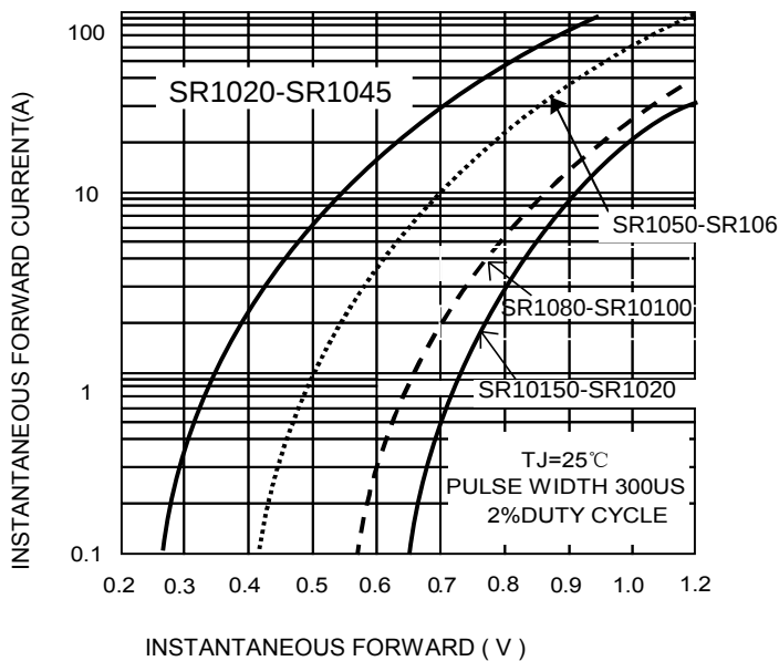
FIG.2-TYPICAL FORWARD CHARACTERISTICS
