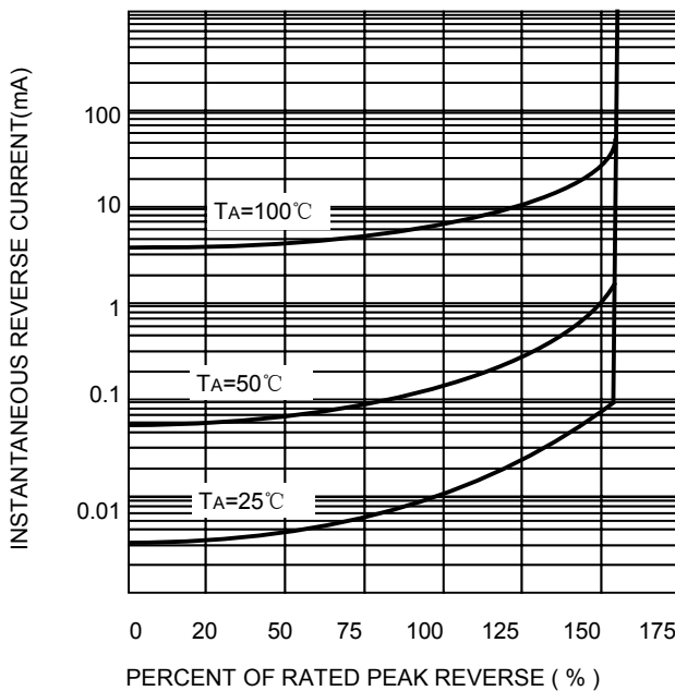
FIG.4-TYPICAL REVERSE CHARACTERISTICS
