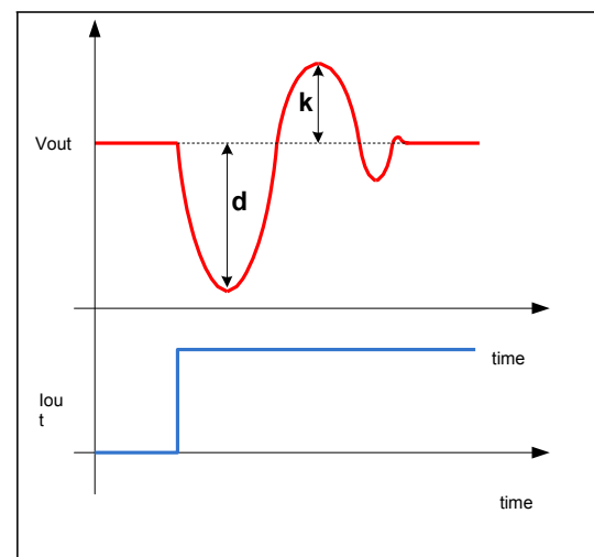
Figure 28 – load step response example and “kick” vs. “kick” definition
