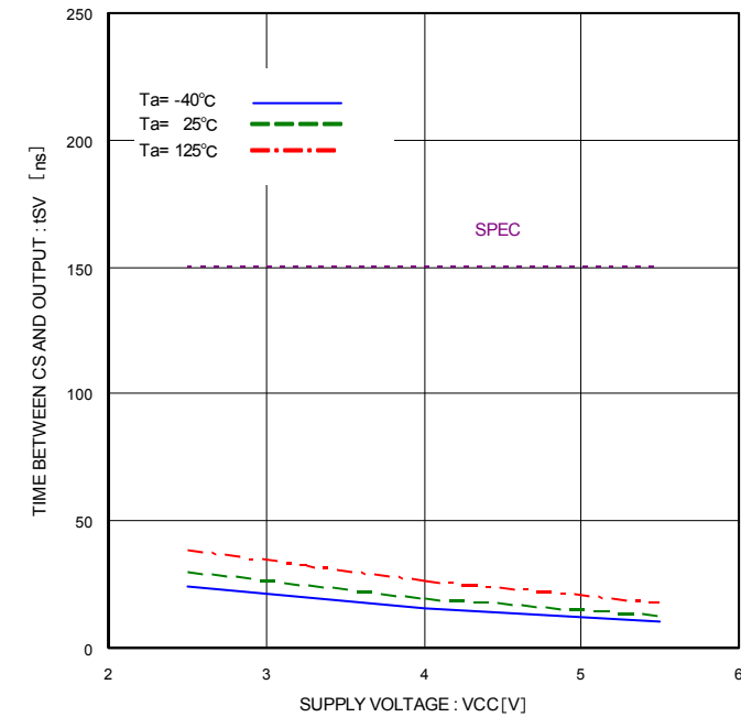
Figure 26 Time Between CS and Output vs. Supply Voltage
