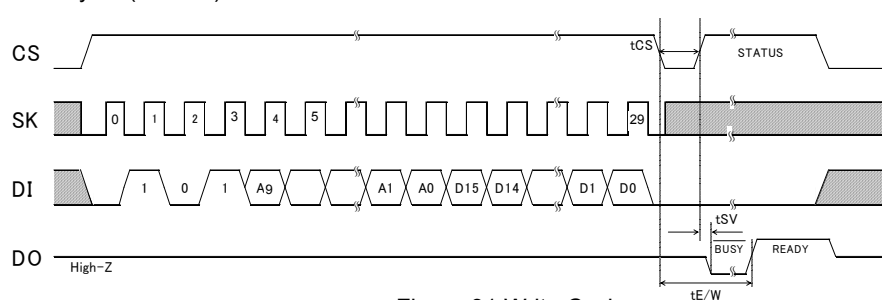
Figure 31 Write Cycle
