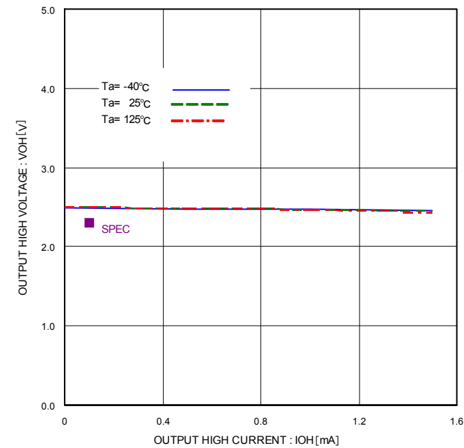
Figure 8 Output High Voltage vs. Output High Current (V CC =2.5V)
