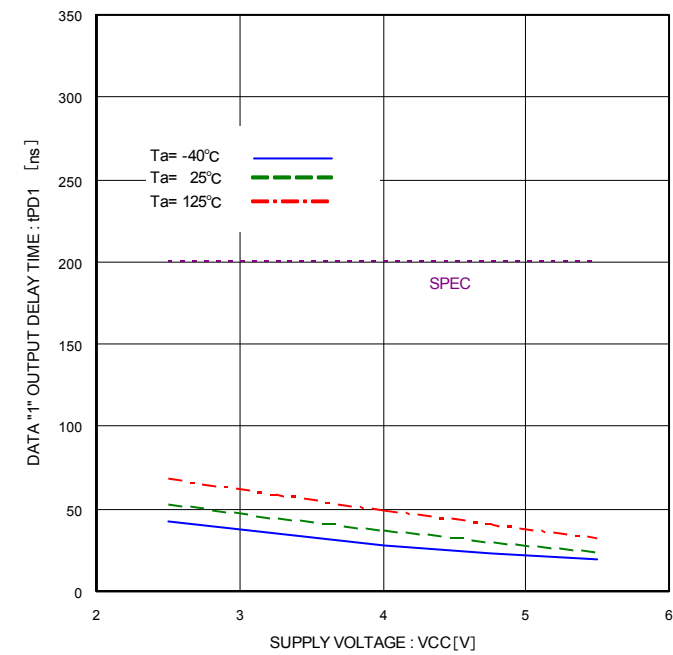
Figure 24 Data "1" Output Delay Time vs. Supply Voltage
