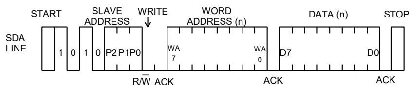
Figure 41. Byte Write
