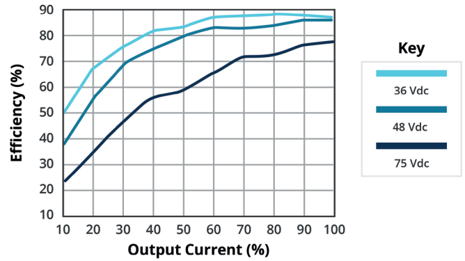
EFFICIENCY VS OUTPUT LOAD PDQ2-D48-D15-S
