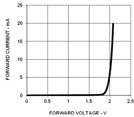
Figure 4: Forward Voltage vs. Current
