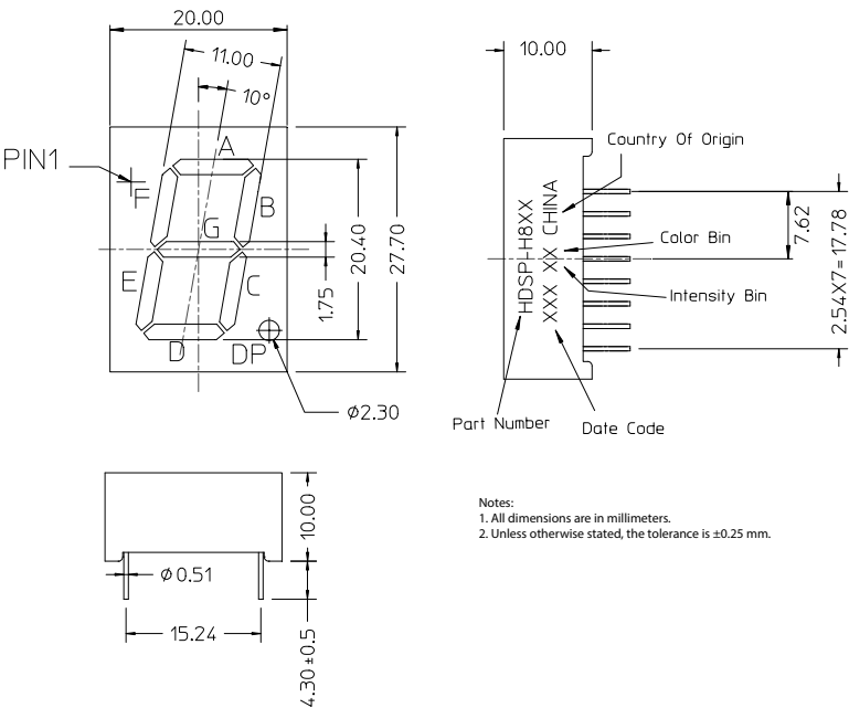
Figure 1: Package Dimension
