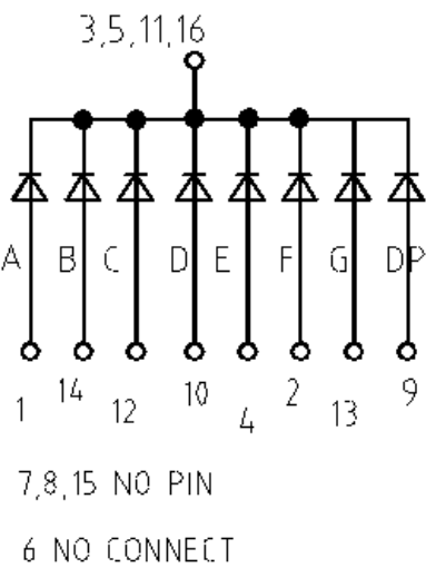
Figure 2: Circuit Diagram
