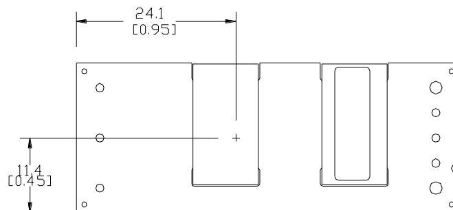
Figure 21. Pick and Place Location.
