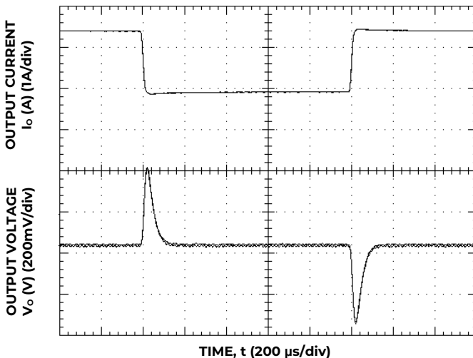
Figure 5. Transient Response to 0.1A/μs Dynamic Load Change from 50% to 75% to 50% of full load, V_{IN}=48V , C_o>100\mu F .
