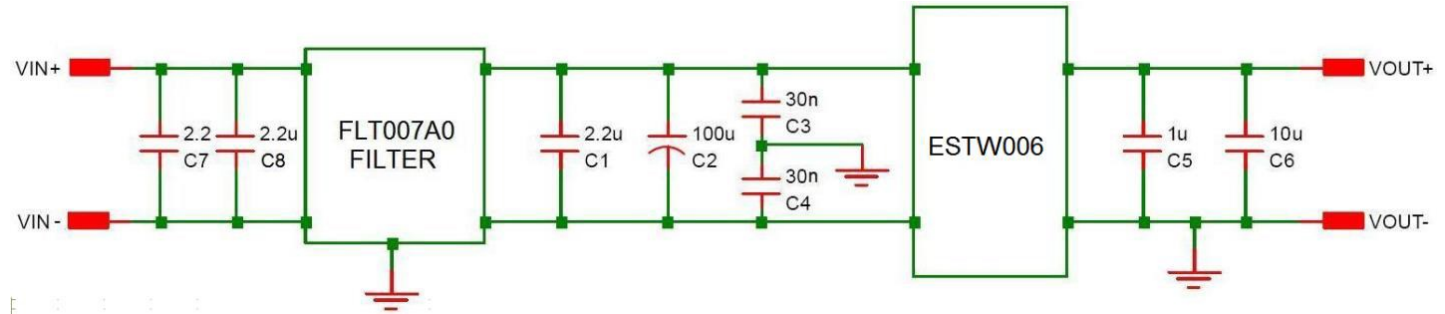
Figure 24. EMC Considerations
