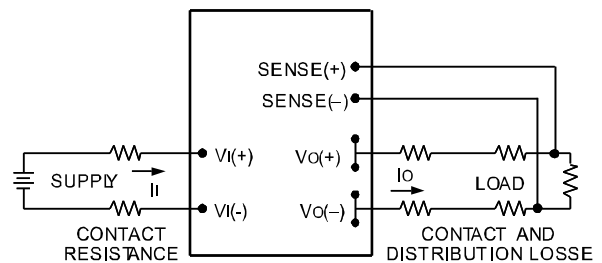
Figure 11. Circuit Configuration for remote sense .
