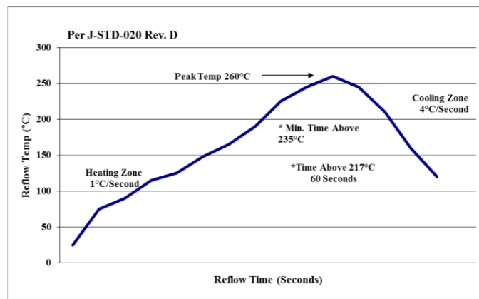
Figure 24. Recommended linear reflow profile using Sn/Ag/Cu solder.
