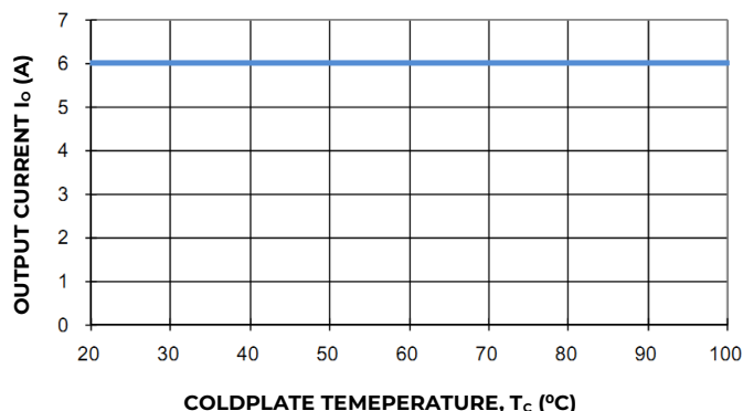
Figure 20. Derated Output Current versus Cold Wall Temperature with Local Ambient Temperature Around Module at 85°C; V_{in} = 48V .
