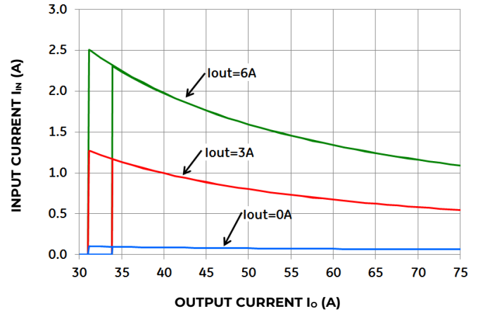
Figure 2. Input Current versus Output Current.
