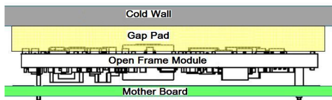
Figure 19. Cold Wall Mounting
