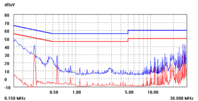
V_{IN} = 48V , I_o = I_{o,max} , N Line Blue= Quasi-peak, Red = Avg
