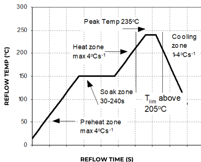
Figure 22. Reflow Profile for Tin/Lead (Sn/Pb) process.
