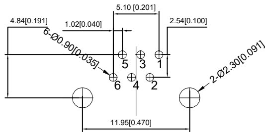
RECOMMENDED PCB LAYOUT VIEWED FROM COMPONENT SIDE
